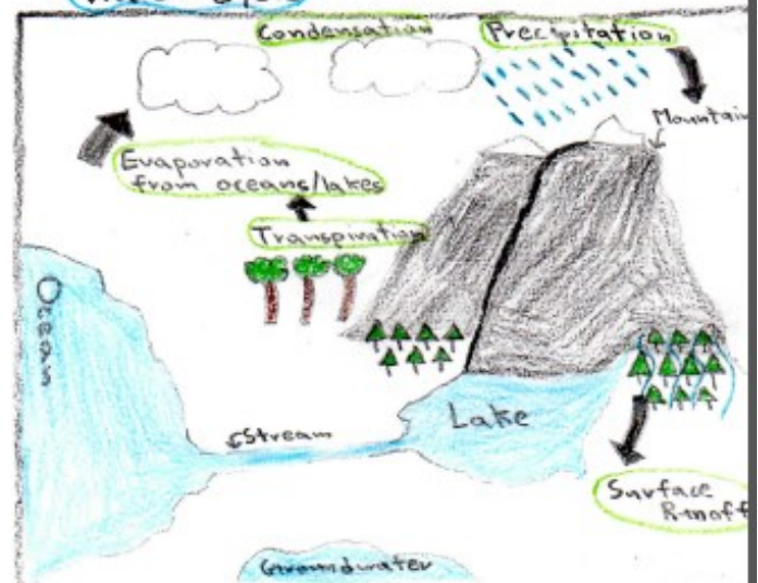
Water Cycle
